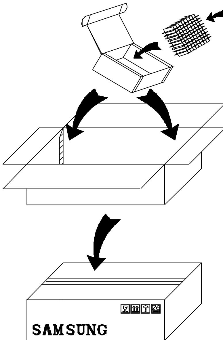
Fig 2. Package Drawing
