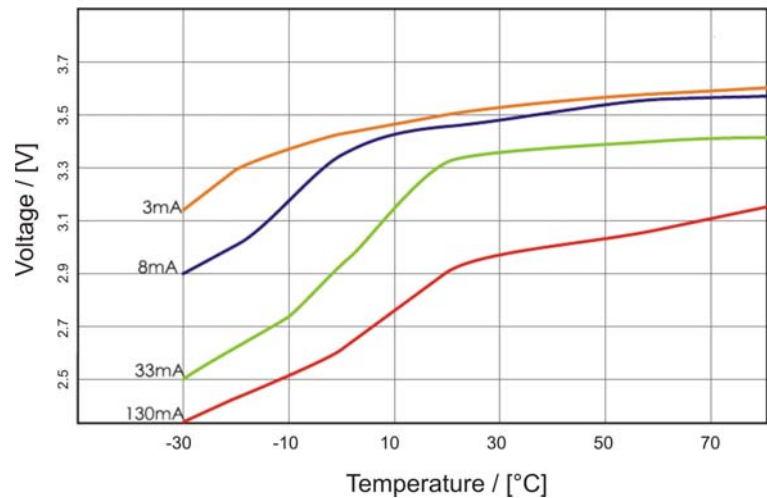
Temperature characteristics
