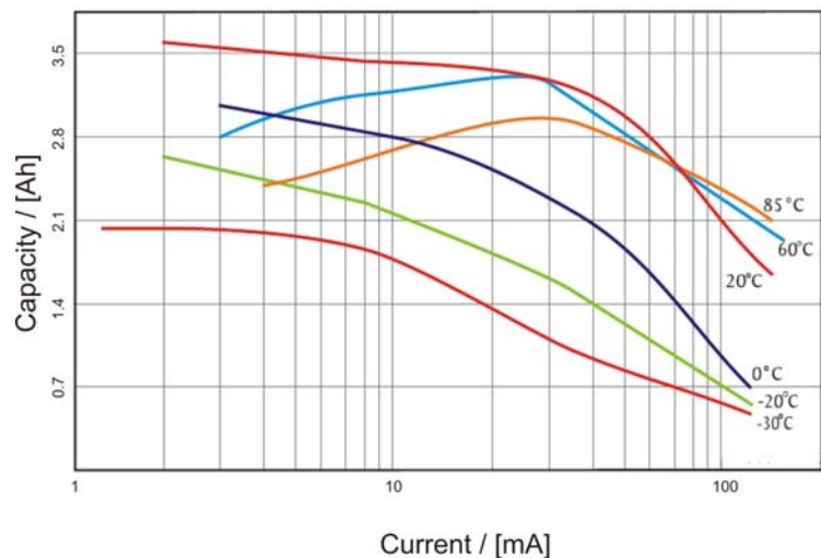
Temperature characteristics
